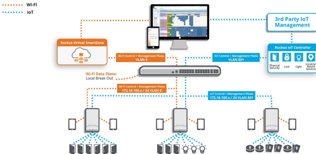
FIGURE 1 Typical Ruckus IoT Deployment
